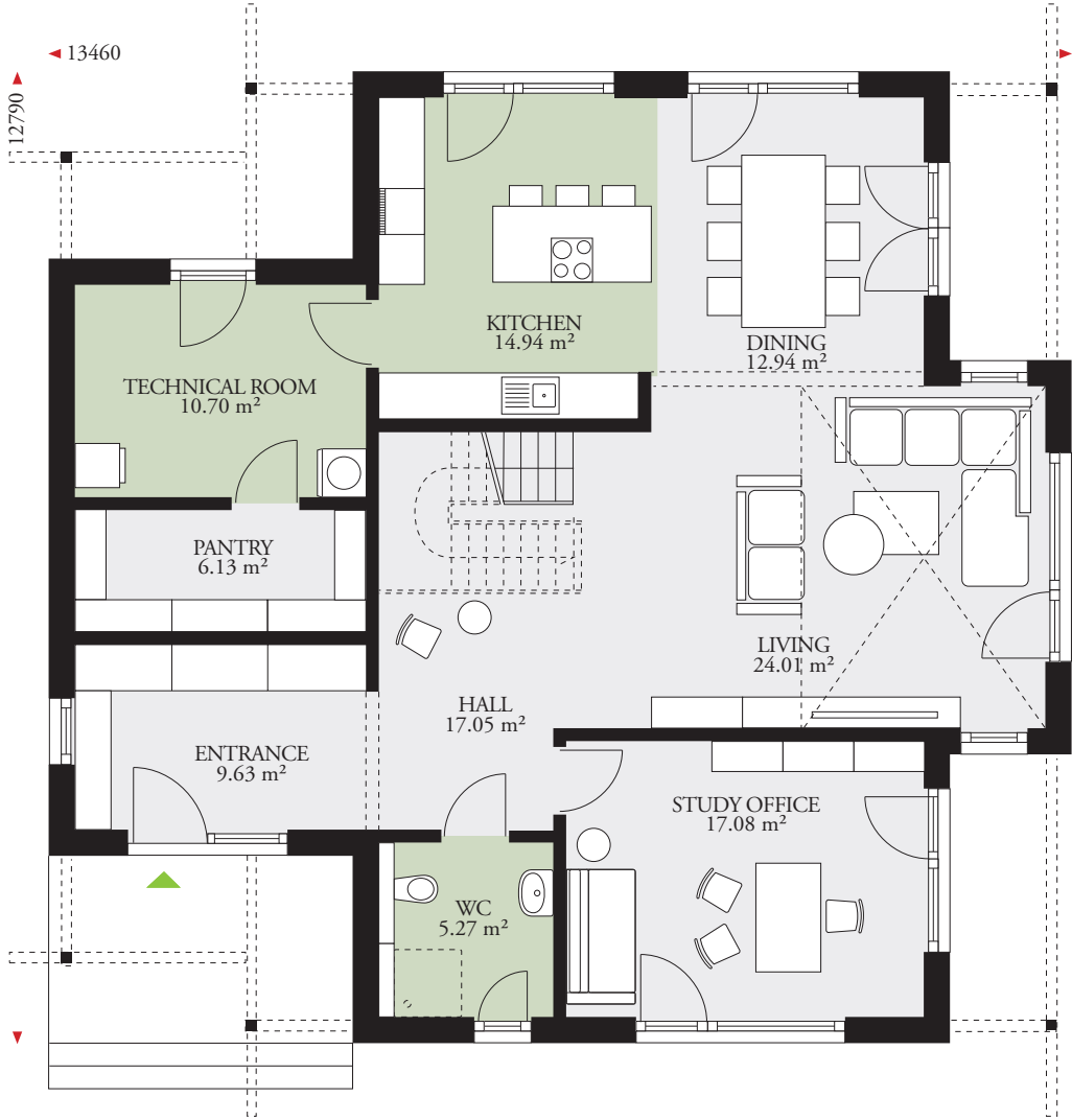
GROUND FLOOR AREA 122.64 m 2 (1,320 sq.ft.)
