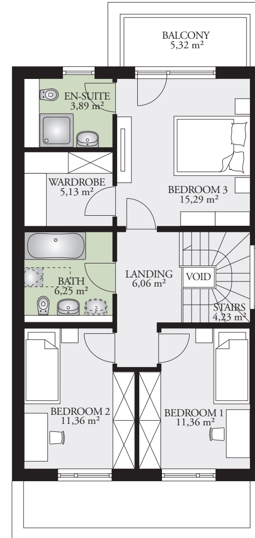
FIRST FLOOR AREA 68,35 m 2 (736 sq. ft)
